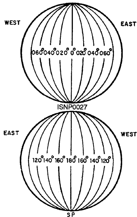
Figure 5-6.—Meridians of longitude.
